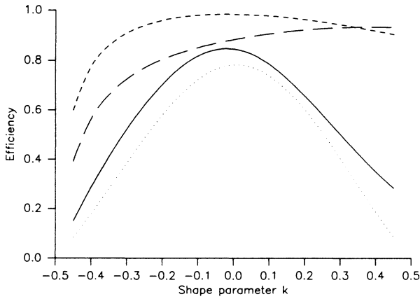
Figure 4. Asymptotic Efficiency of PWM Estimators of Parameters of the GEV Distribution: — \hat{k} ; - - - \hat{\alpha} ; ···· \hat{\xi} ; ····· overall efficiency (i.e., ratio of determinants of asymptotic covariance matrices of ML and PWM estimators).
