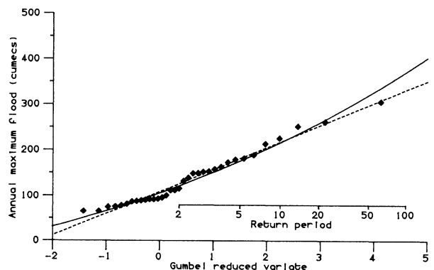
Figure 5. Distributions Fitted by the Method of PWM to 35 Annual Maximum Floods of the River Nidd: — GEV distribution; - - - Gumbel distribution.
